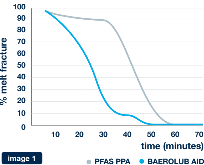
Time to clear with BAEROLUB AID
